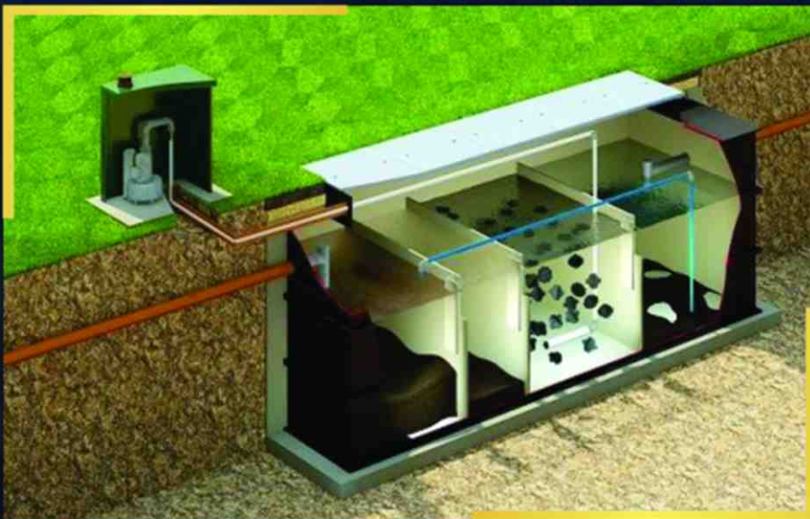
Sewage Facility
